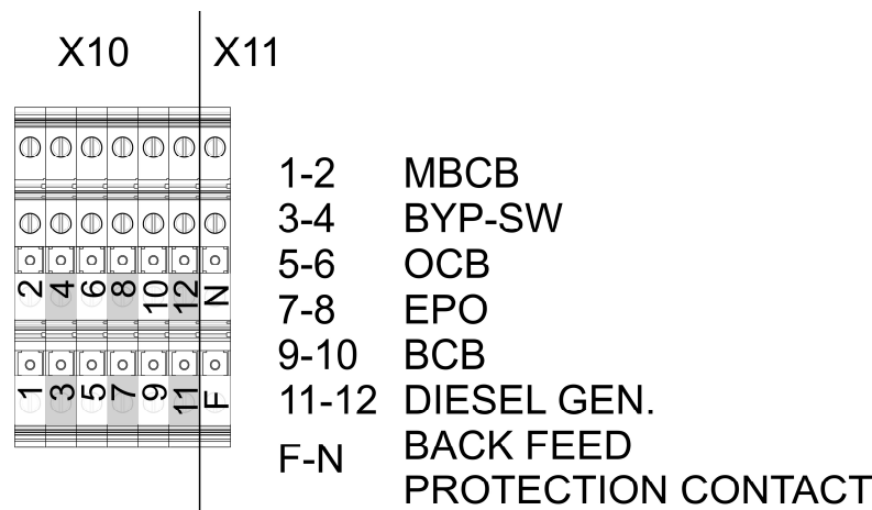
Picture 7 – Auxiliary terminals of INGENIO MAX 400-500 kVA
