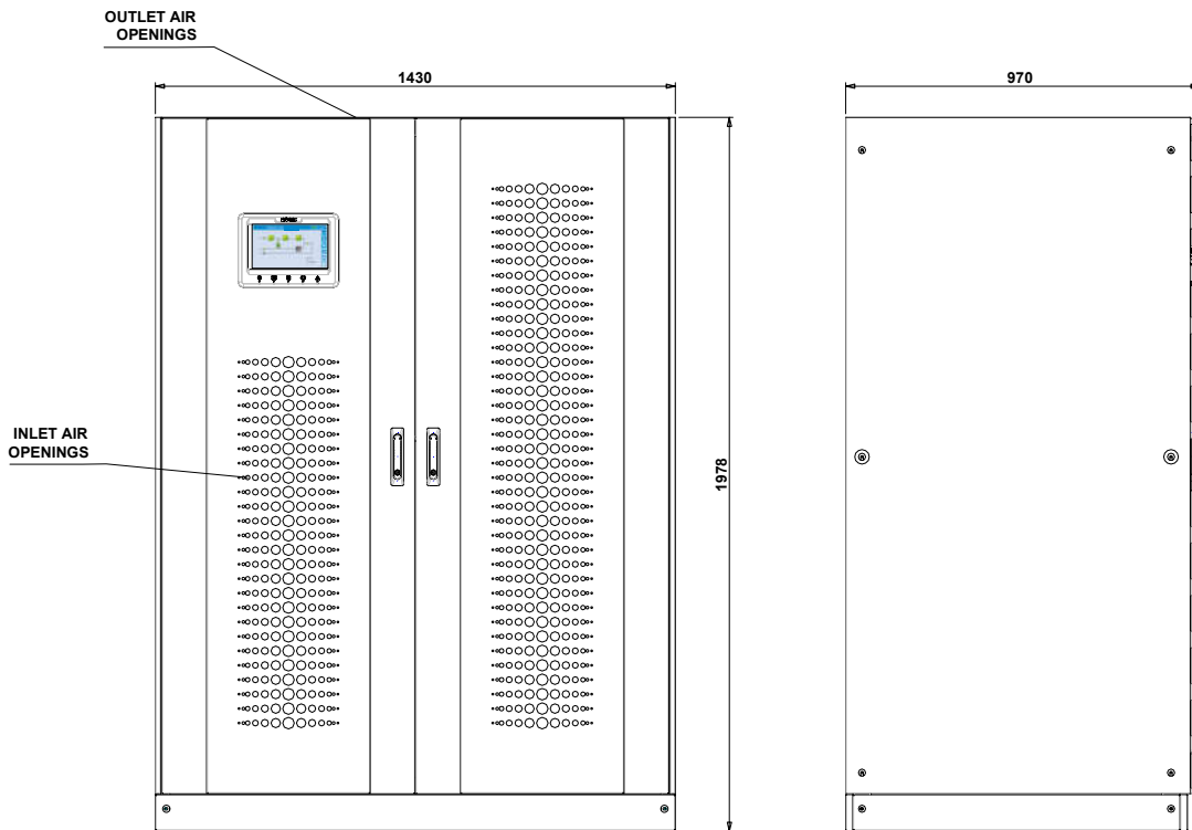
Picture 4 – Overall dimensions
