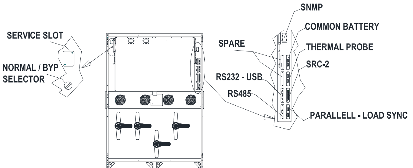
Picture 8 – Position of the serial interfaces of INGENIO MAX 400-500 kVA
