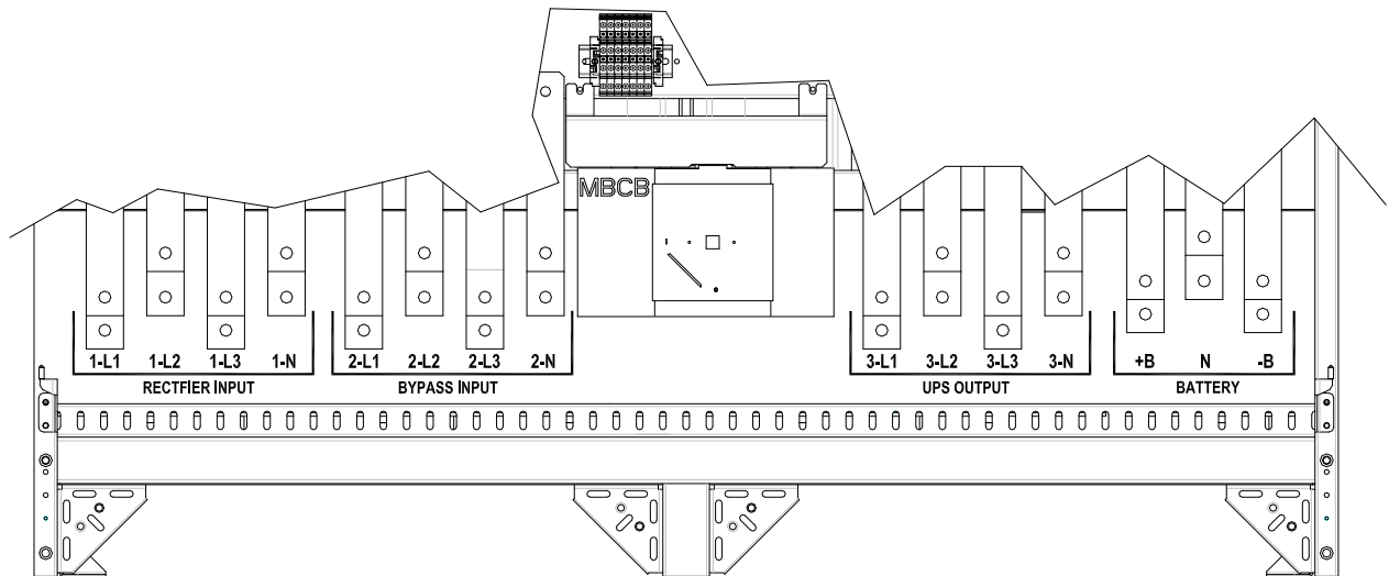
Picture 6 – Terminal board INGENIO MAX 400-500 kVA
