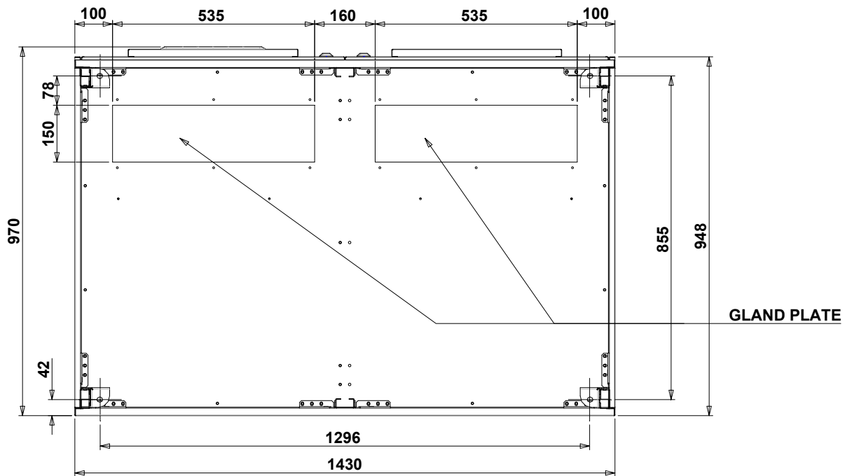
Picture 3 – Base plan
