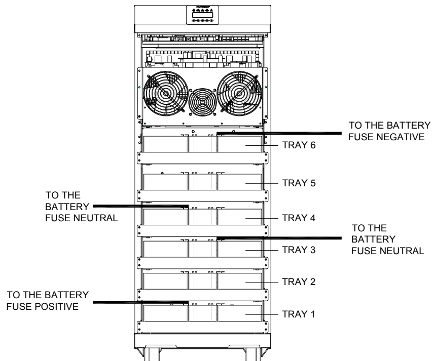
Picture 12- 60 x 9Ah 12V battery connection tray front view
