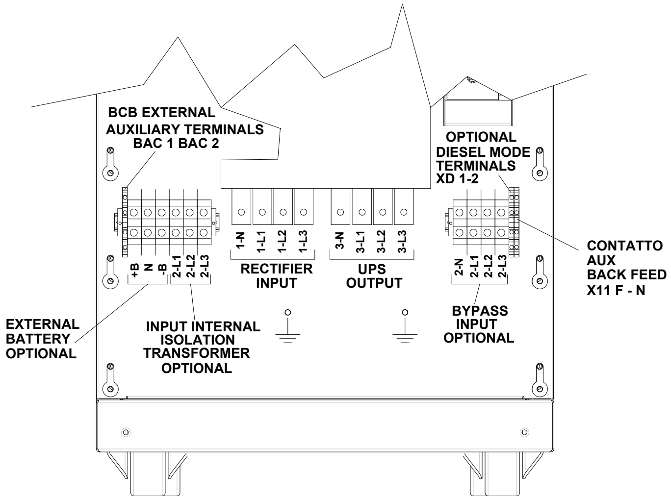
Picture 7 – Terminal board INGENIO PLUS 40 kVA
