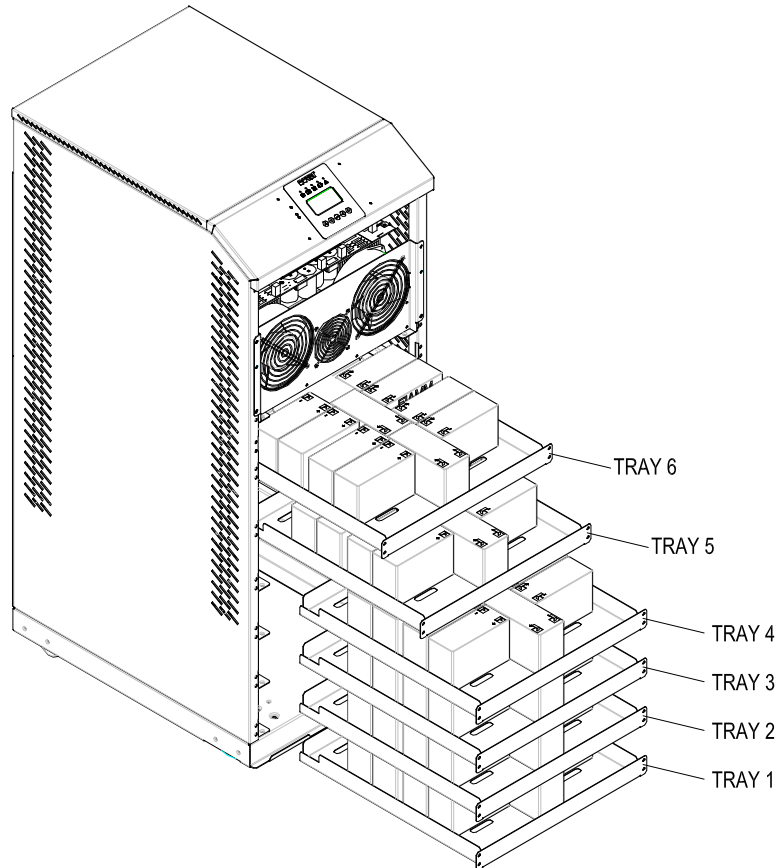
Picture 9 - Trays 60 x9Ah 12V battery lateral view
