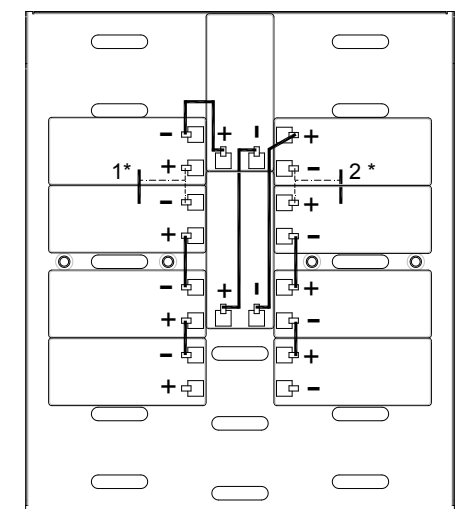
Picture 9 - Trays 60 x9Ah 12V battery lateral view
