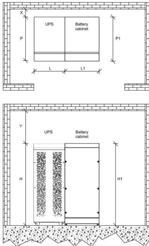
Picture 5 – Minimum distances from the walls
