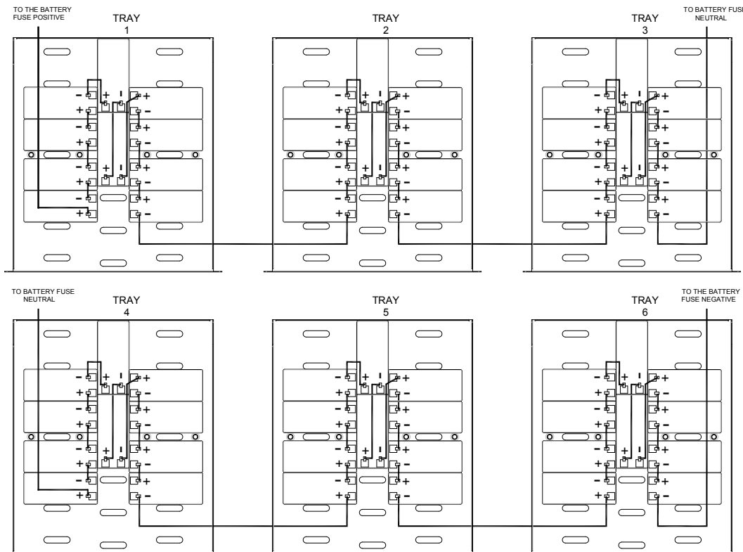
Picture 11 - 60 x9Ah 12V battery connection tray top view
