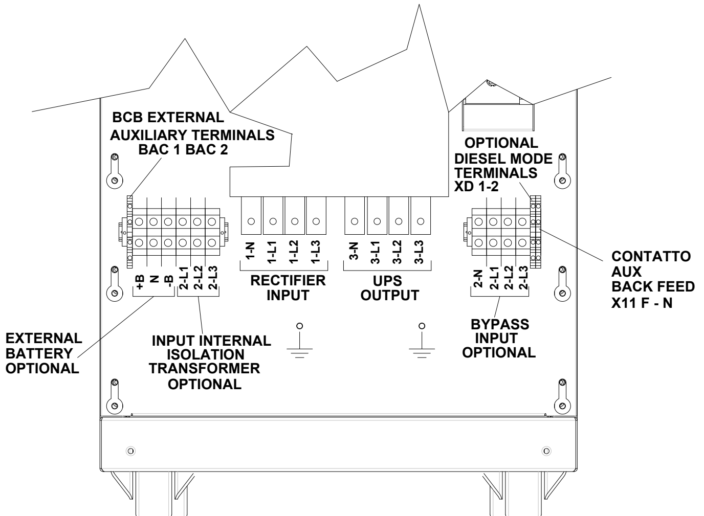
Picture 6 – Terminal board INGENIO PLUS 30 kVA
