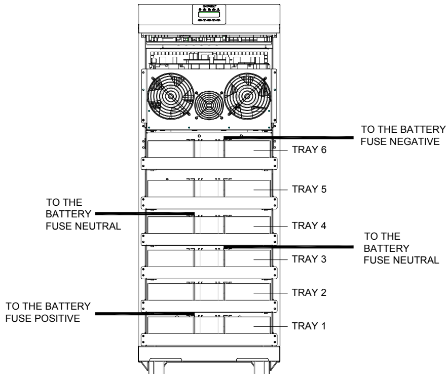
Picture 16 - 60 x12Ah 12V battery connection tray front view
