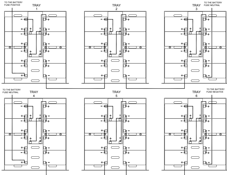
Picture 15 – 60 x 12Ah 12V battery connection tray top view
