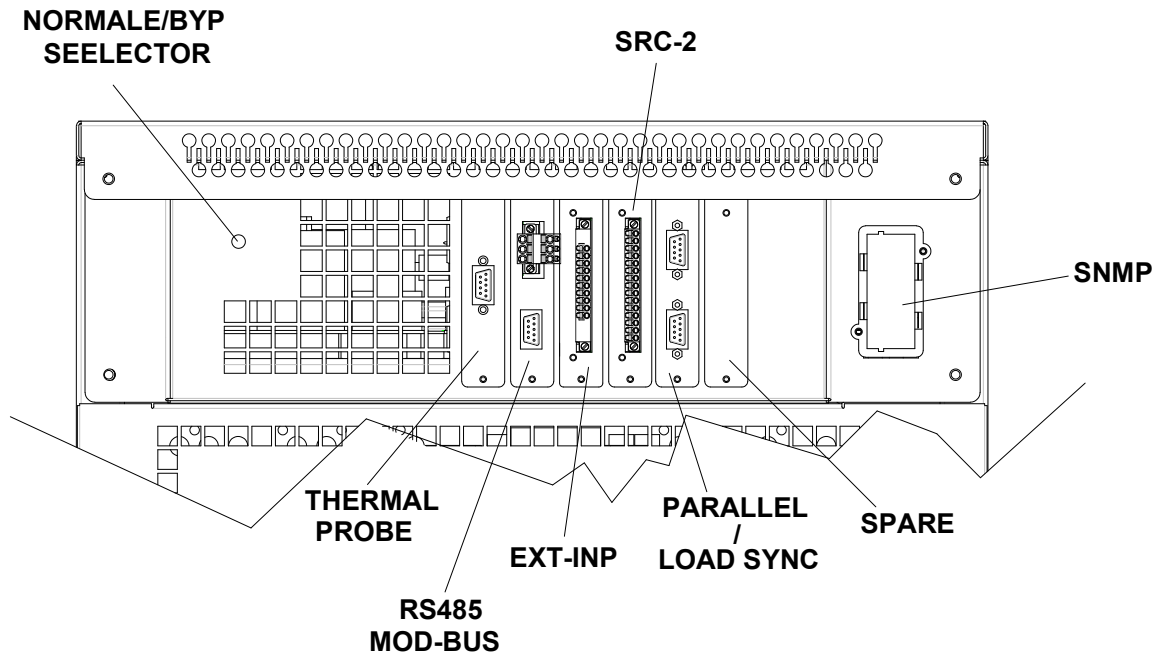
Picture 17 – Position of the serial interfaces of INGENIO PLUS 30÷40 kVA
