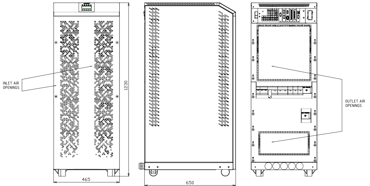
Picture 4 – Overall dimensions
