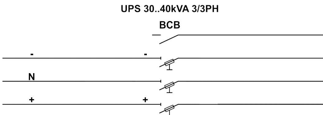
Picture 8 – Cabling of BCB fuse holder
