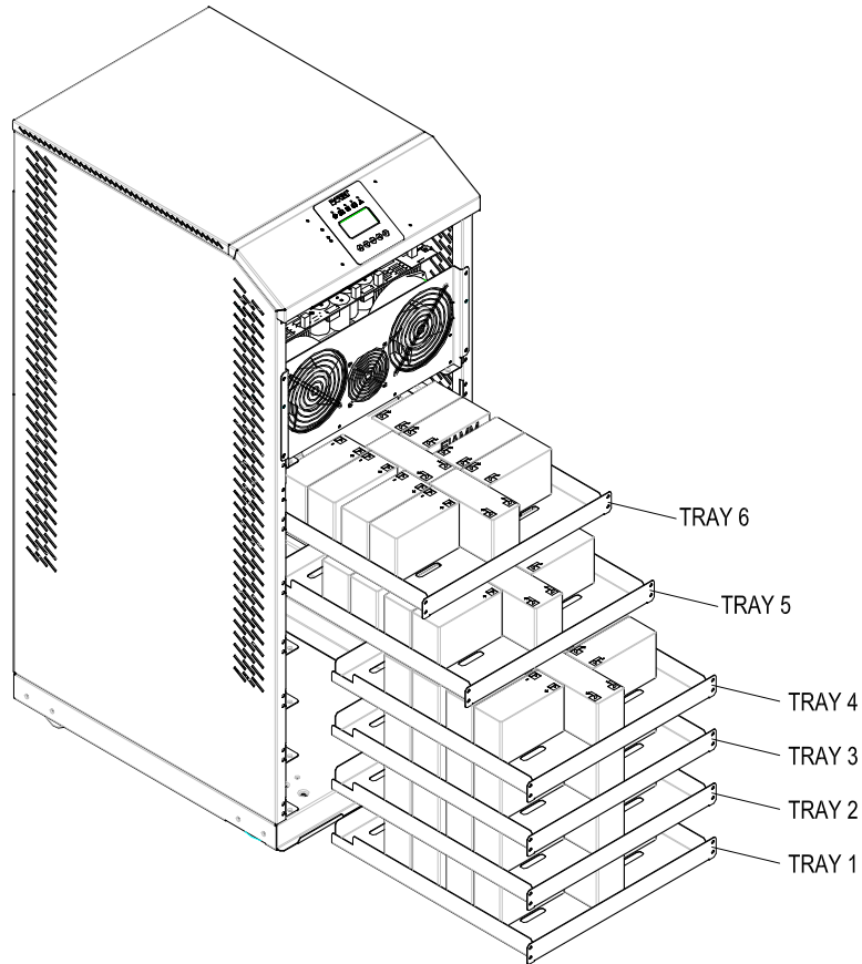
Picture 13 - Trays 60 x 12Ah 12V battery lateral view
